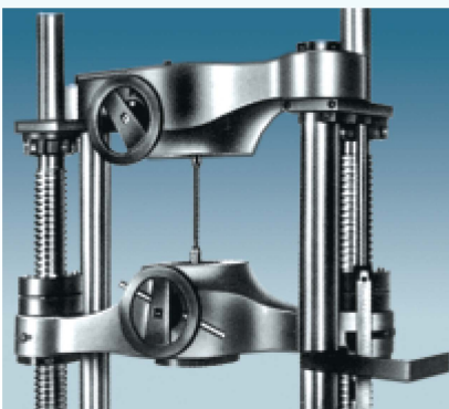
Tension Test
