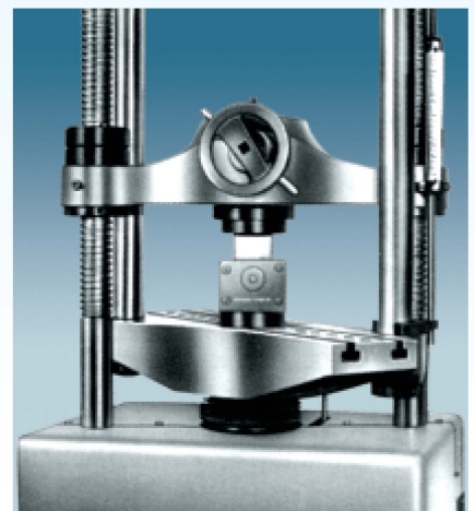
Shear Test
