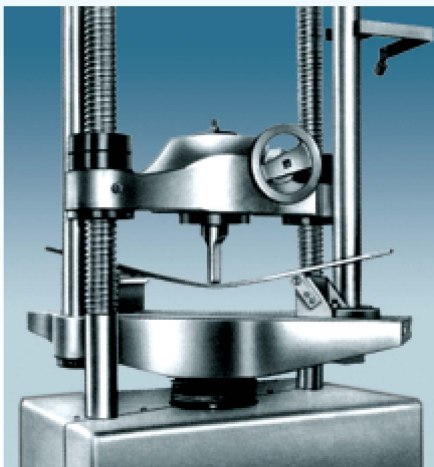
Transverse Test
