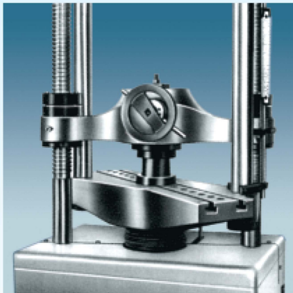
Compression Test
