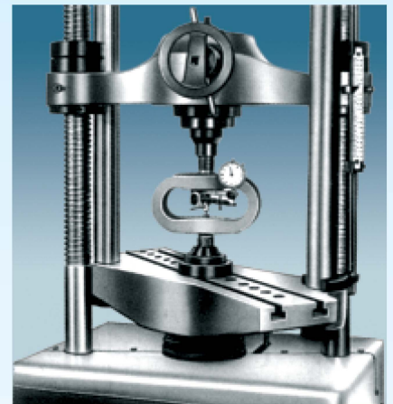
Calibration of Machine with providing Ring
