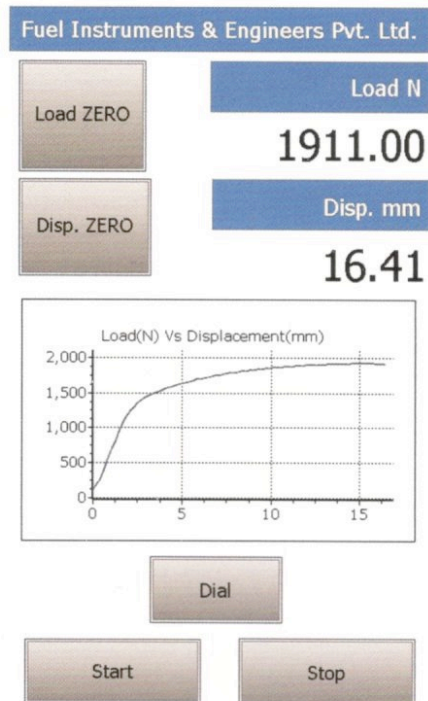
Real time Graph with load & displacement
